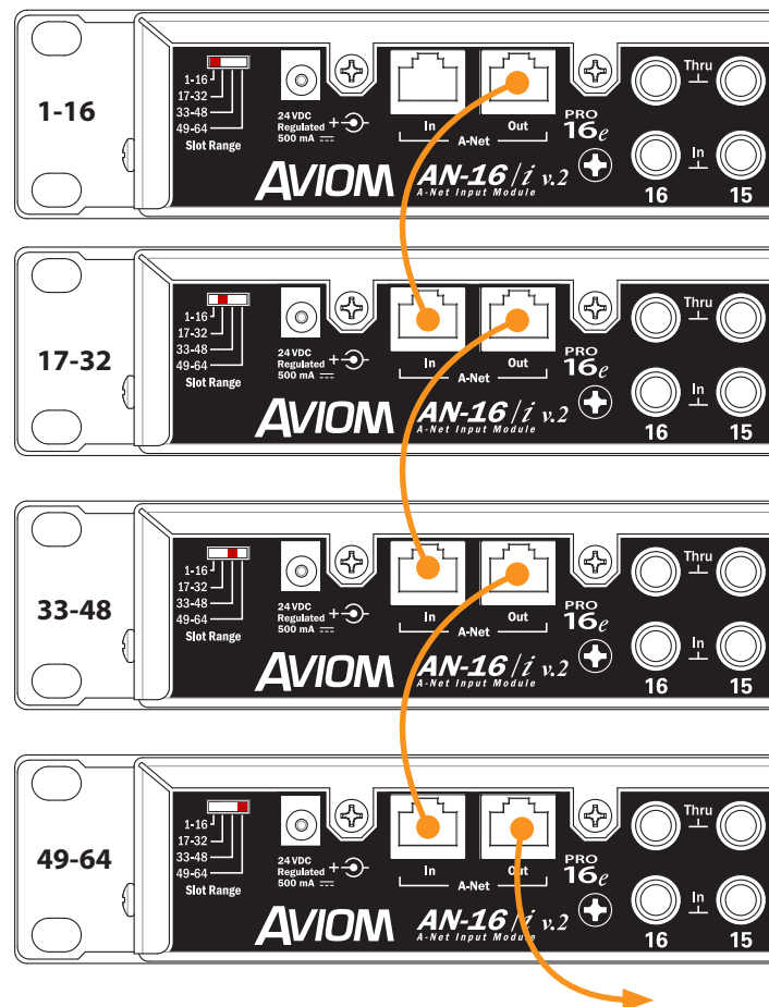
Slot Range switches for each input device in at system are shown. A legacy Pro16 device may be substituted for the first bank of 16 channels.
